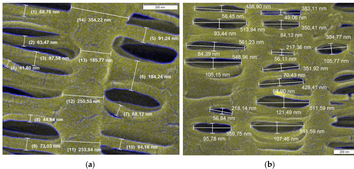
Figure 4. Evaluation of collector diameter (a) and pore size (b) from SEM images using Stream Motion software.
