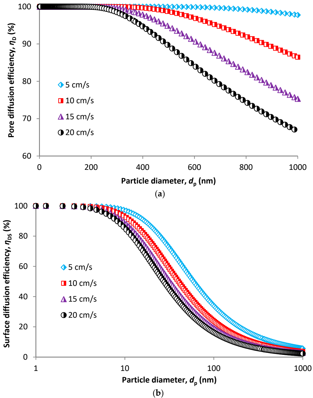
Figure 12. Collection efficiency due to diffusion in pores (a) and on the membrane surface (b).
