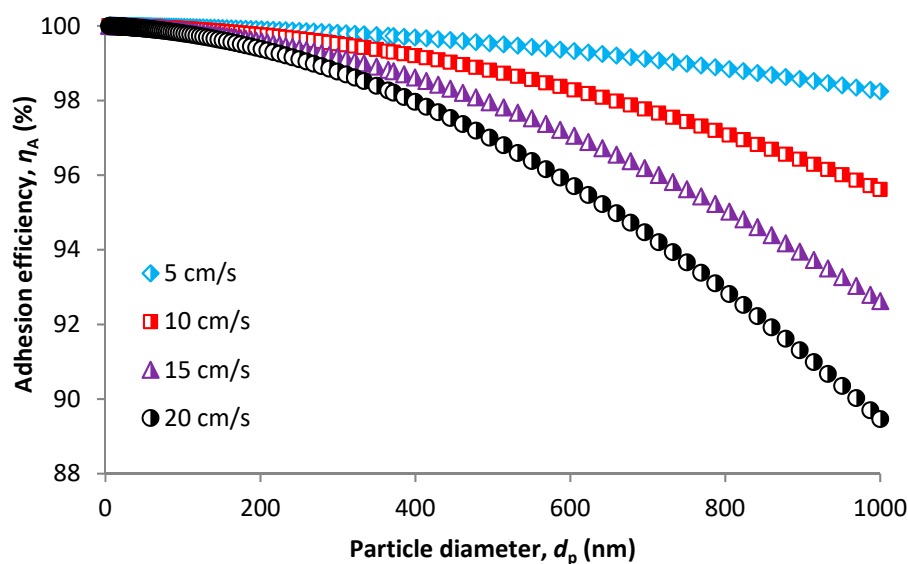
Figure 8. Collection efficiency due to the adhesion effect.
