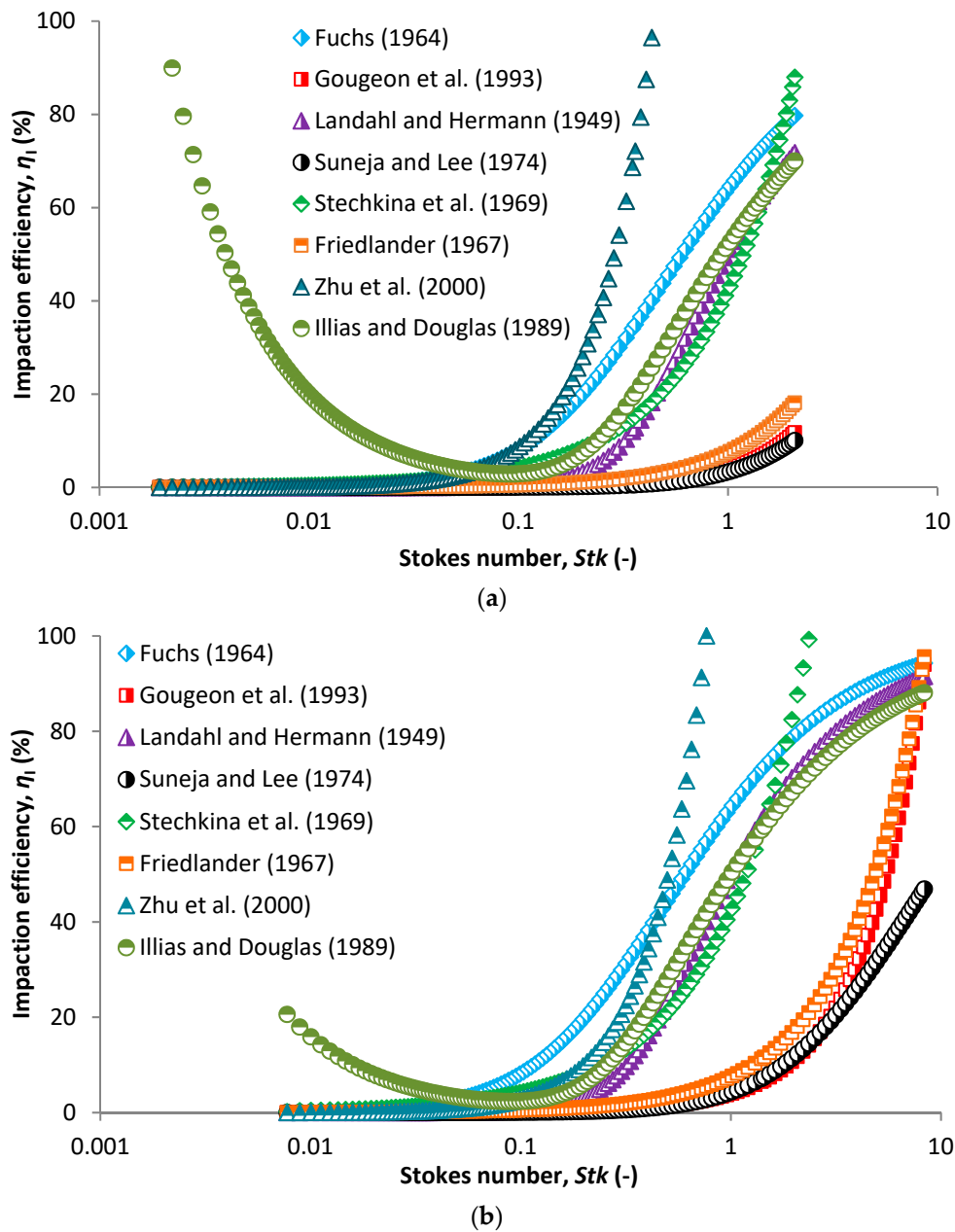
Figure 5. Comparison of impaction efficiency based on different models and airflow velocity of 5 cm/s (a) and 20 cm/s (b) in relation to Stokes number.
