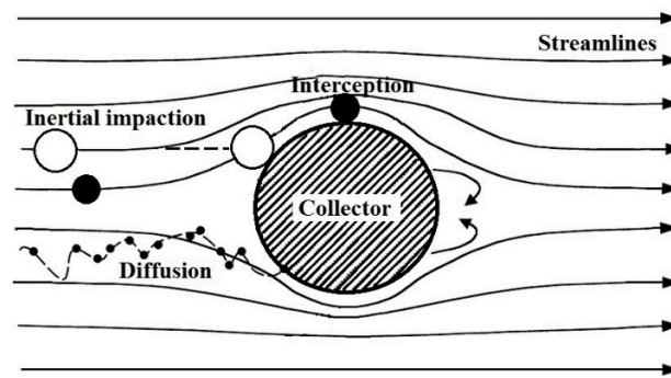
Figure 2. Schematic presentation of individual collection mechanisms at a single collector.
