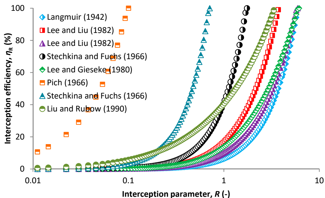
Figure 6. SCE due to interception based on various models in relation to interception parameter.
