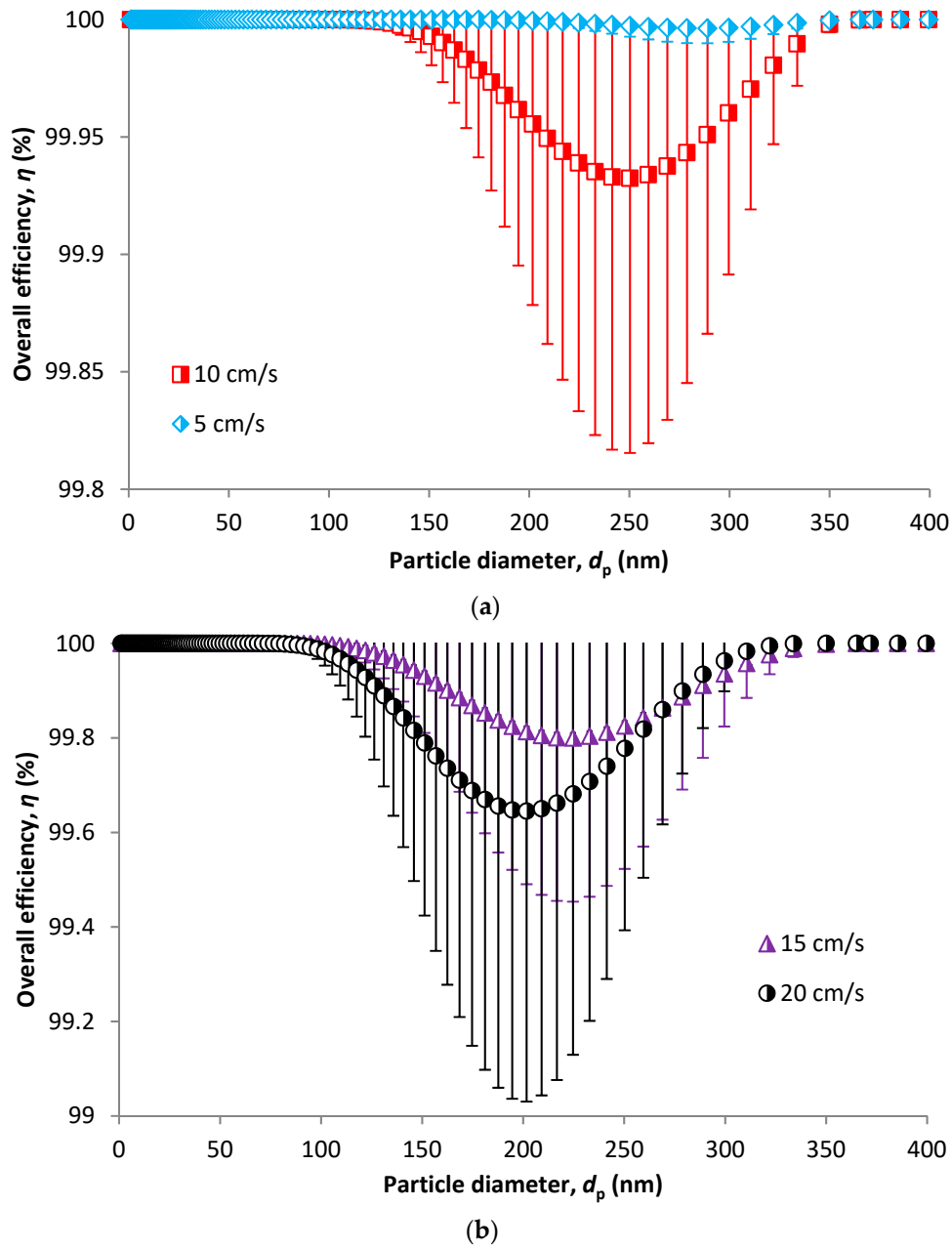
Figure 13. Overall efficiency in relation to particle size based on CPM model for a velocity of 5 and 10 cm/s (a) and 15 and 20 cm/s (b).
