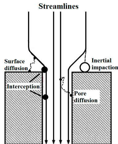
Figure 3. Schematic filtration mechanisms involved in separation on a CPM.
