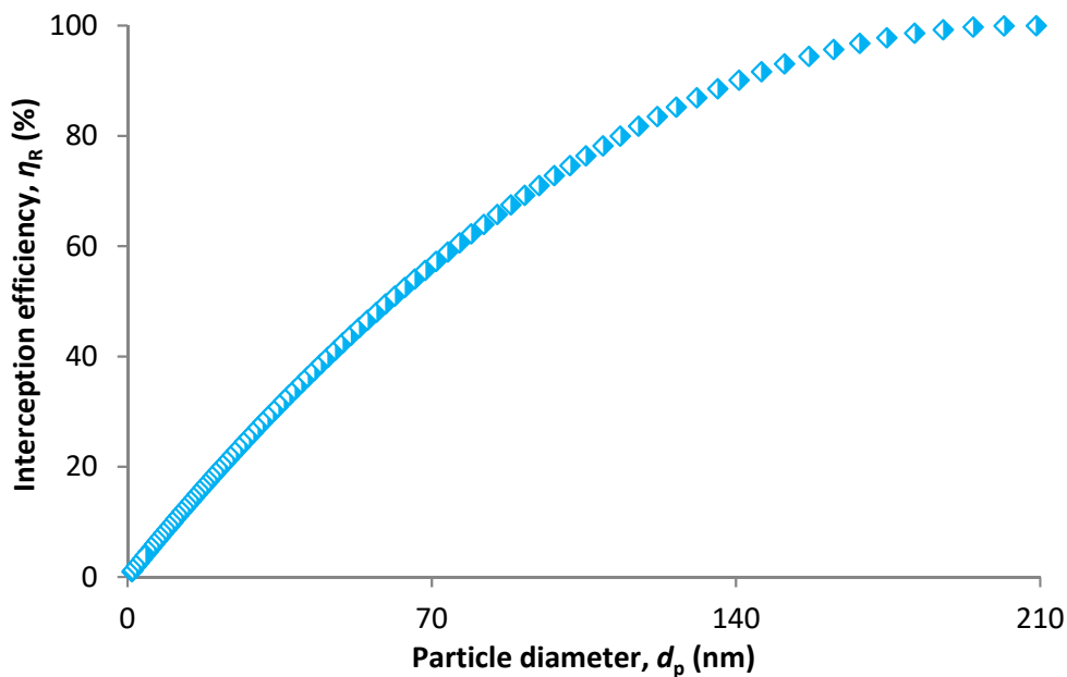
Figure 11. Interception efficiency based on CPM model.
