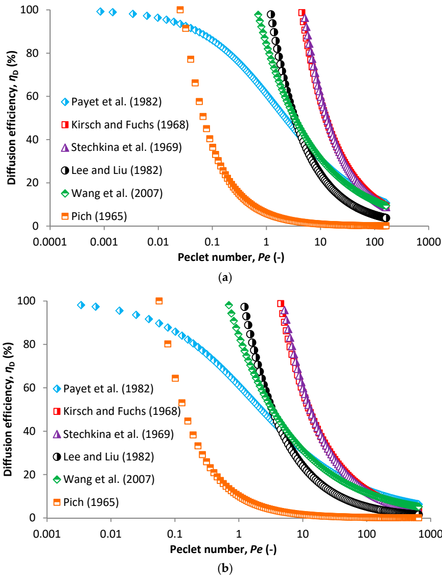
Figure 7. Comparison of SCE due to diffusion mechanisms based on different models for an airflow velocity of 5 cm/s (a) and 20 cm/s (b) in relation to the Peclet number.
