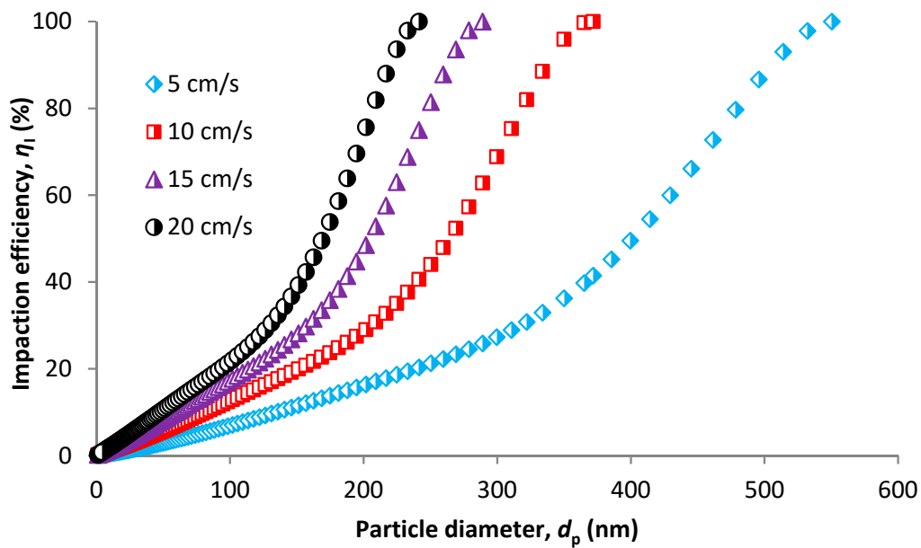
Figure 10. Impaction efficiency based on CPM model.
