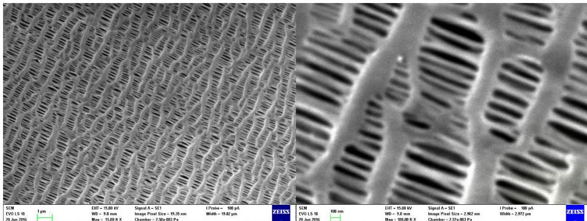
Figure 1. Polypropylene HFM pore structure.
