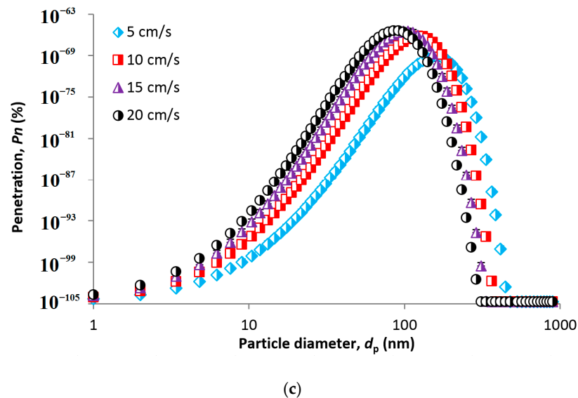
Figure 9. Single collector efficiency (a), overall filter efficiency (b) and overall penetration (c).
